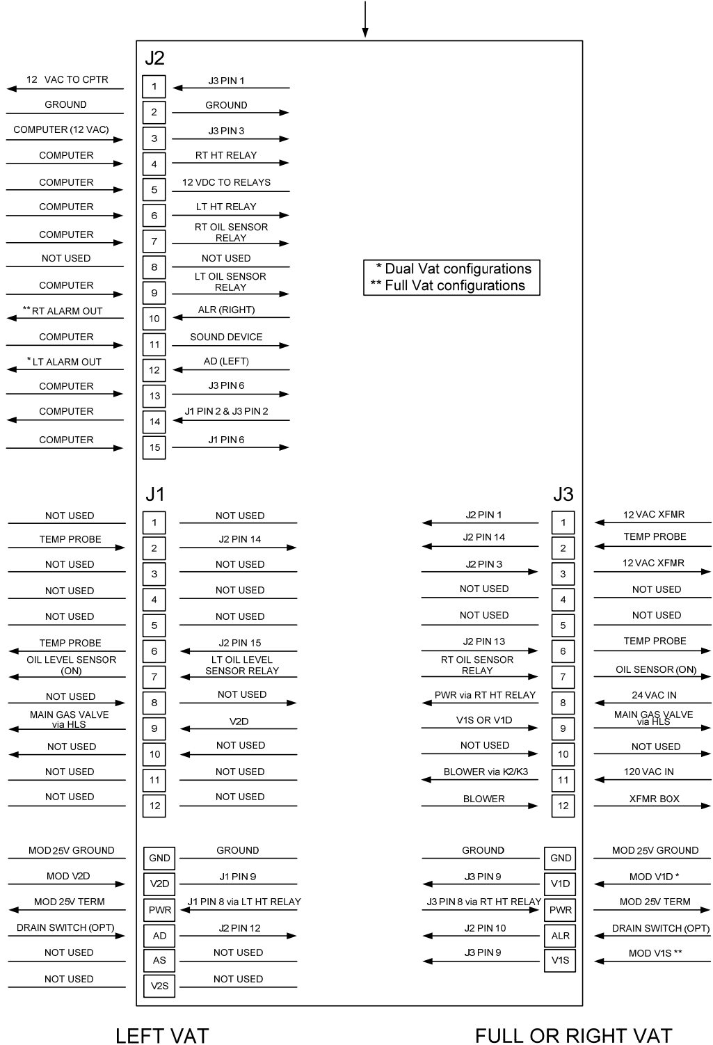
CURRENT FLOW THROUGH INTERFACE BOARD 106-6706 (SMT LOV SERIES APPLICATION)
